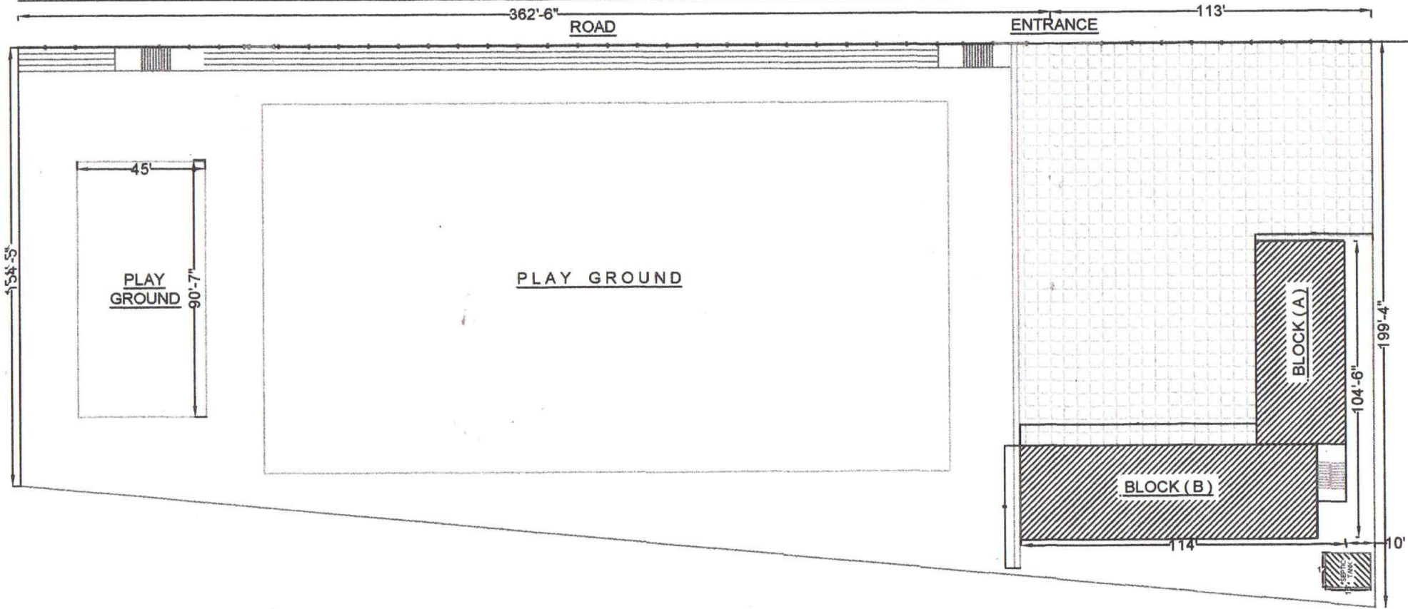
SITE PLAN OF PROPOSED STAFF QUARTER FOR SERA MEY SCHOOL.
